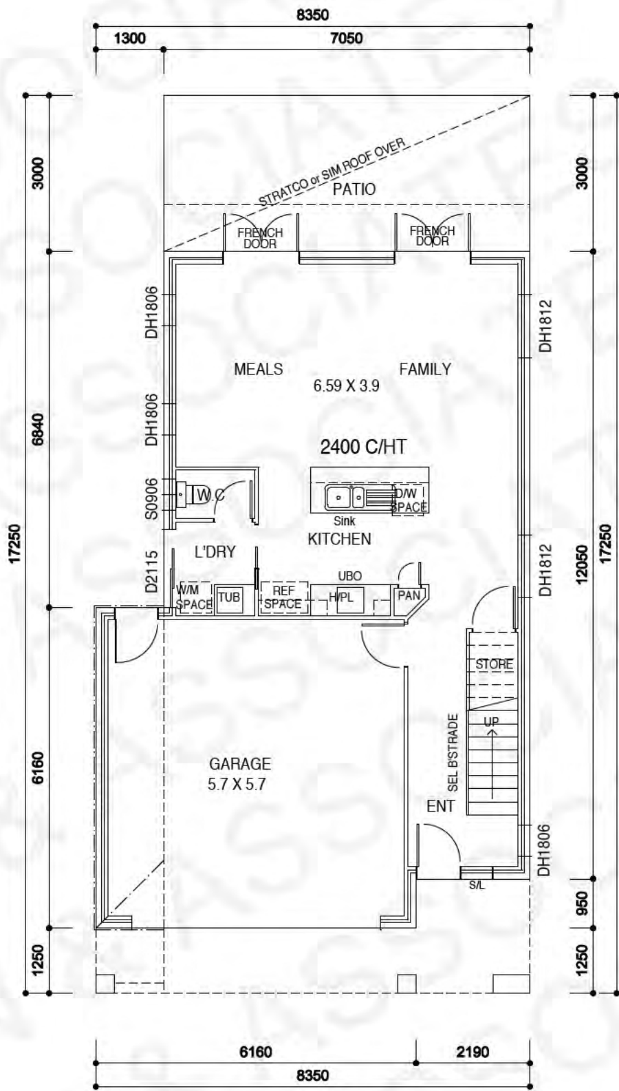
LOWER FLOOR PLAN WILSFL MADD14
