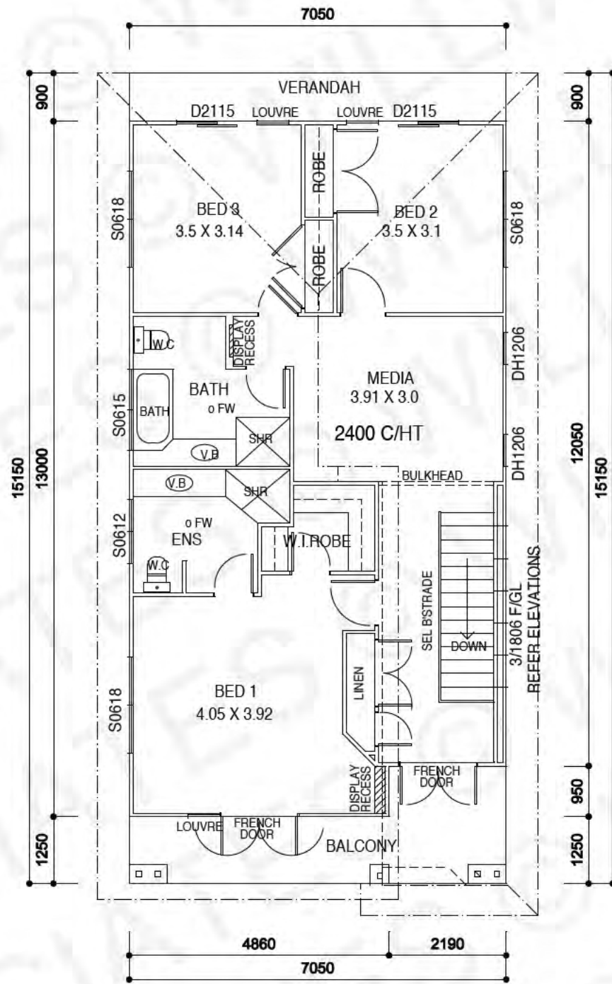
UPPER FLOOR PLAN
